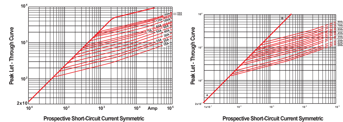
Peak Let - Through Curve - JR30 type
