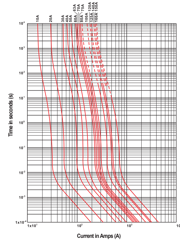
Time-Current Curves - JR60 type
