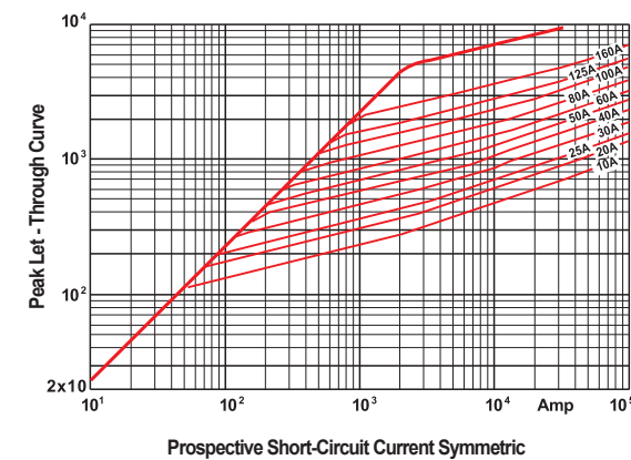
Peak Let - Through Curve - JR60 type
