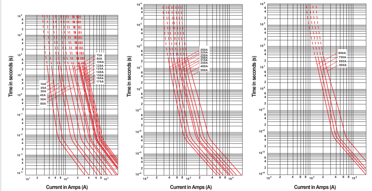
Time-Current Curves - JR30 type
